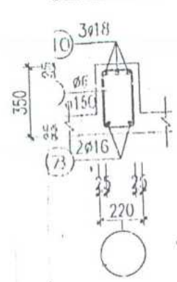
ẮT 7-7 (8-8)
