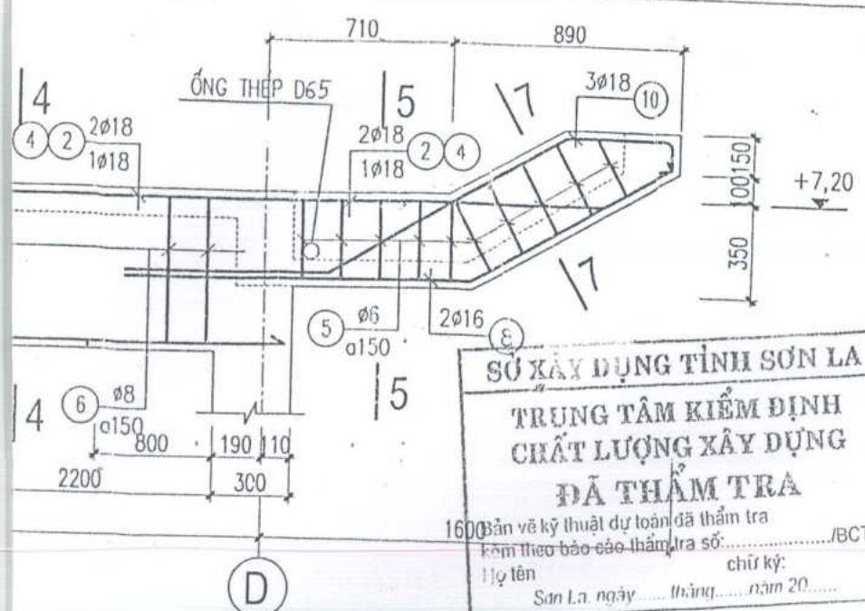
CẮT 7-7 (8-8)
