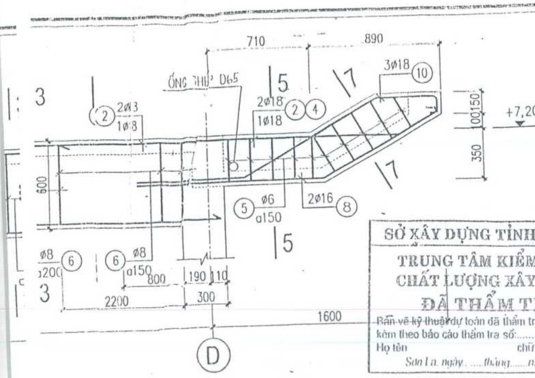
ẮT 7-7 (8-8)
