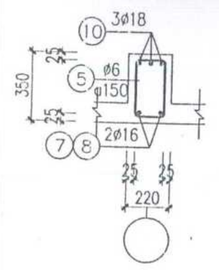
CẮT 7-7 (8-8)
